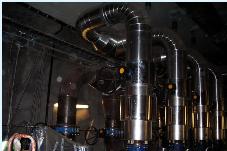
Hornsberg-Stockholm District Cooling (Scandinavia)
